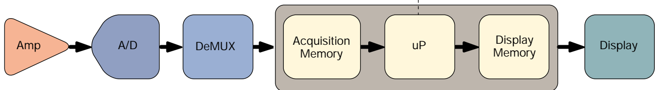
► Figure 2. Digital Storage Oscilloscope, Serial Processing Technology 1982.
